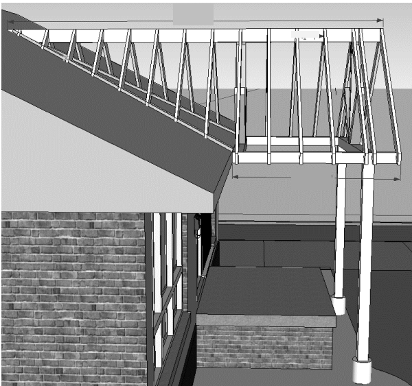
FIGURE 2: JOISTS WITH DROPPED BEAM - DECK ATTACHED AT HOUSE
